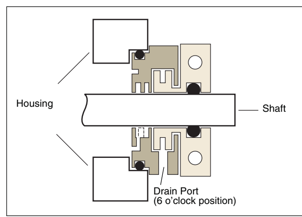
Figure 8-3. Proper Installation
