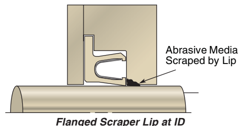
Flanged Scraper Lip at ID
