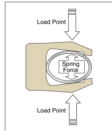
Figure 2-16. Installed State
