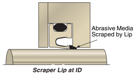
Scraper Lip at ID
