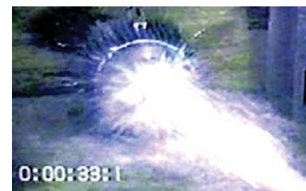
IP X6 Water Exclusion Testing
