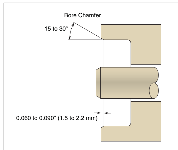
Figure 6-2. Housing Profile
