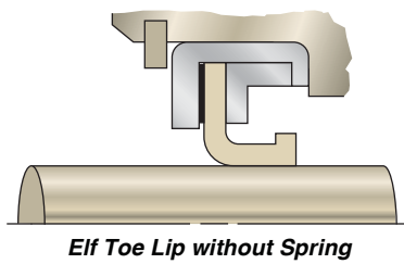
Elf Toe Lip without Spring
