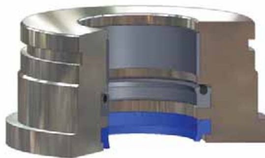
Rod sealing system comprised of WN wear ring, Type B PolyPak and SHD wiper
