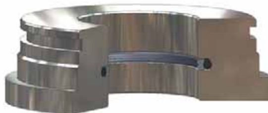
OR installed on Rotary Shaft Gland
