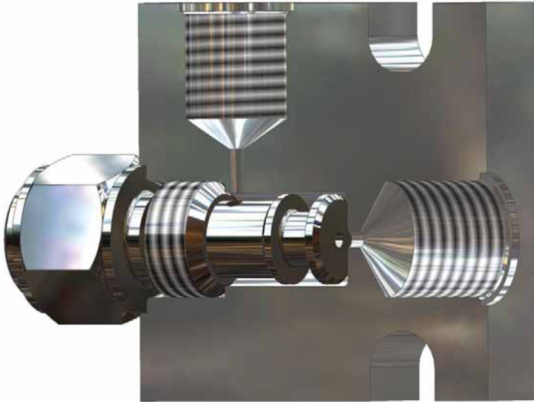
Figure 4-13. Cartridge Valve
