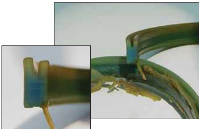
Figure 2-5. Extrusion damage
