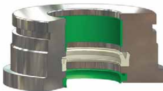
AY installed in Rod Gland
